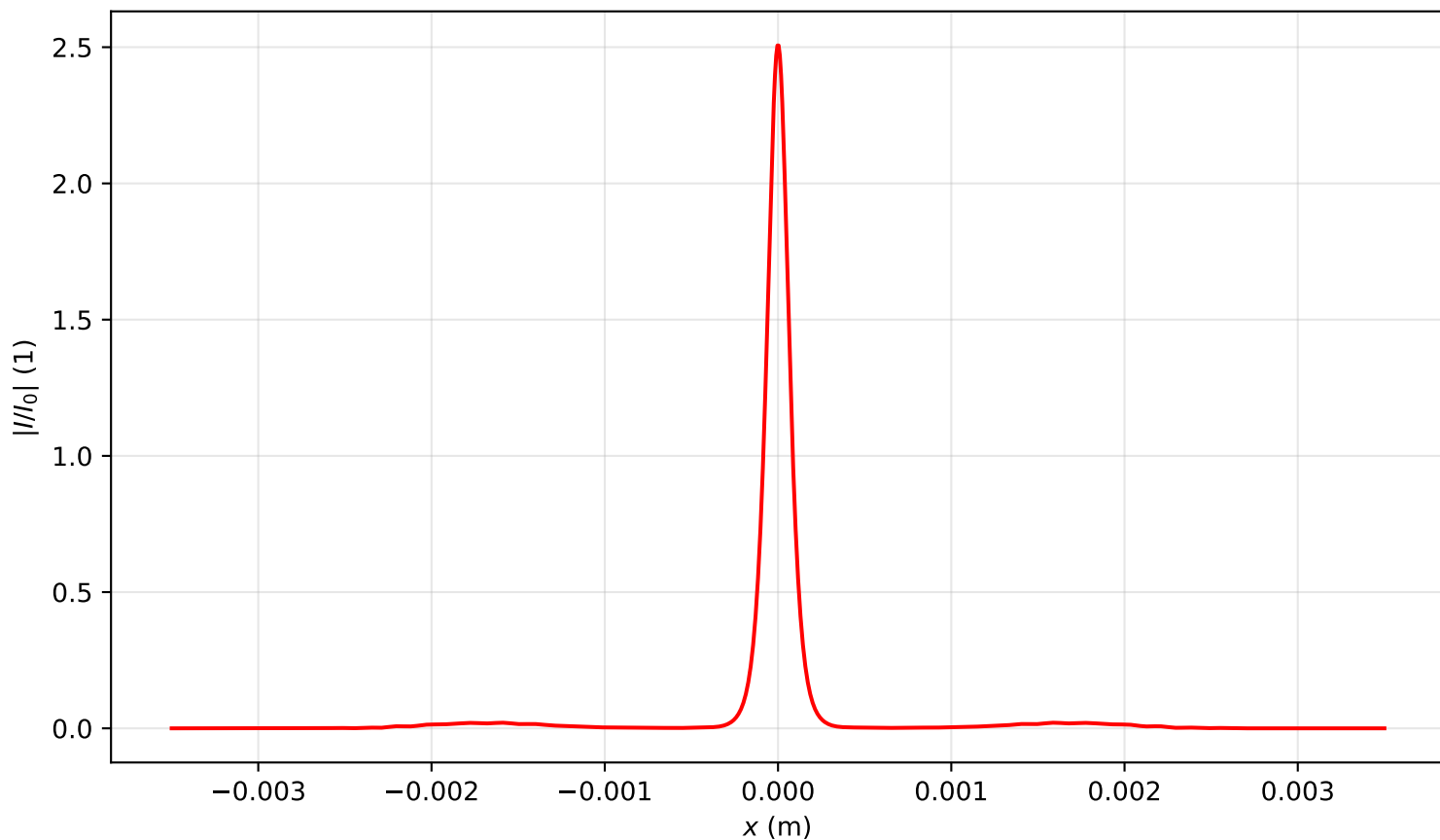
Intensity profile I(x, y = 0, z = 1.274)/I_0 , P_{in}=6.0P_{cr} , artificial time
